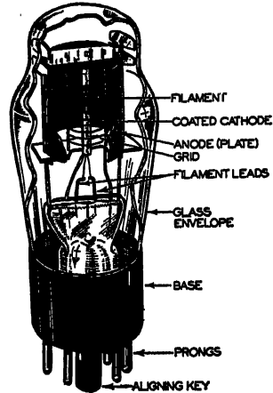
Cutaway diagram showing construction of a typical radio tube.
